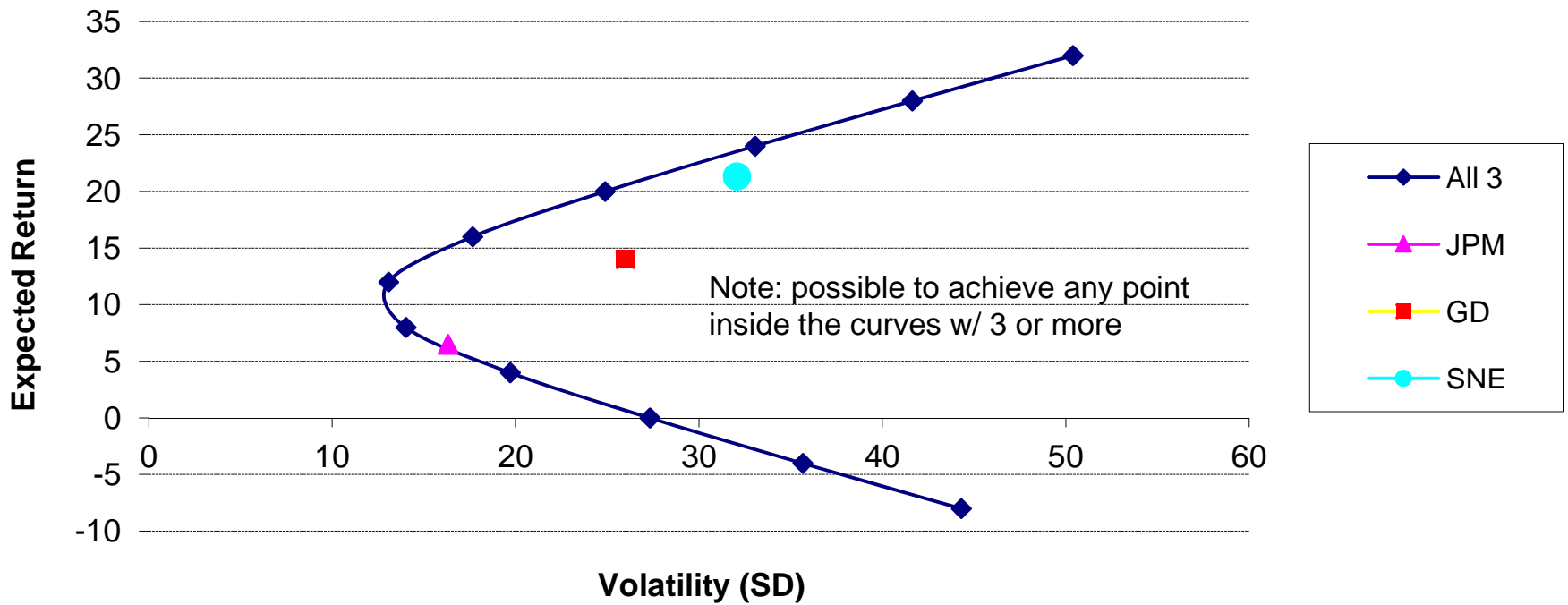
Graph #7d: Porfolios of 3 stocks (long and short) w/ corr = 0
