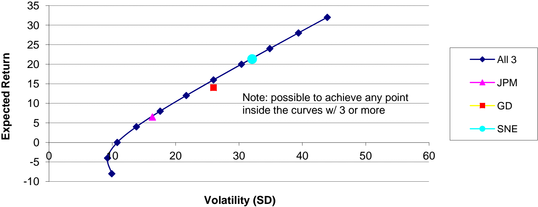
Graph #7a: Portfolios of 3 stocks (long and short) w/ Corr = .95
